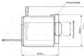
WWH0802 DIMENSIONS
