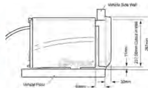
WWH0802 DIMENSIONS
