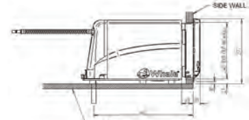
WWH1302 DIMENSIONS
