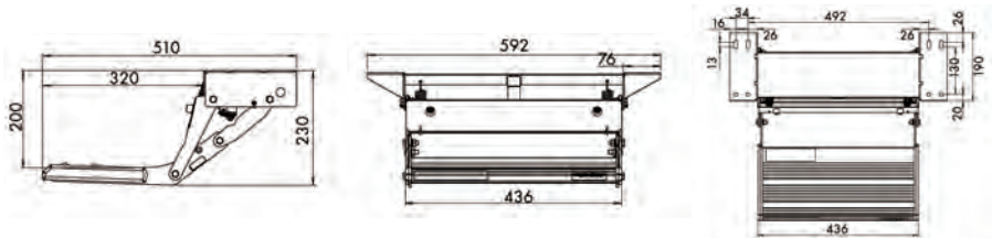
ES1075044 Electric single step standard
