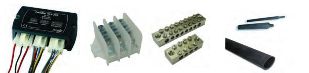
ETB3x5 Multi spade isolated distribution connector block. Provides 3way x 5 connectors Earth terminal block Nickel plated brass ETB4 Earth Block 4way ETB8 Earth Block 8way EHS5164 Heat shrink tubing 6.4mm un-shrunk black polyolefin Pack contains 5 x 1mtr lengths.
