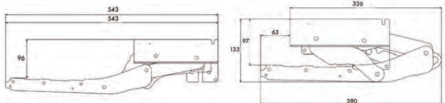
ES1075155 Electric step 550MM (9.1KG)
