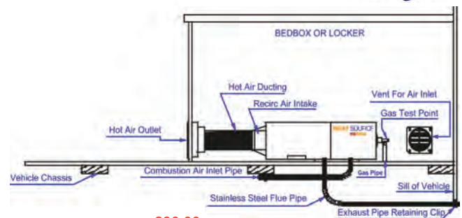
COMPACT UNDERFLOOR BLOWN AIR HEATER - See Page 57 for details
