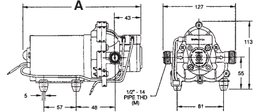
A = 197mm for 7 ltr models, A = 226mm for 10 ltr models. Approximate measurements for all pumps
