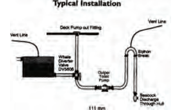
Typical Installation
