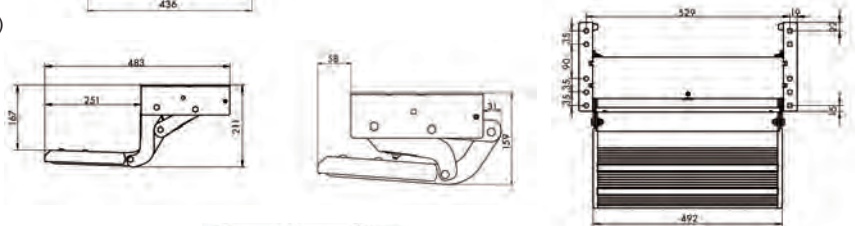
MS1247450 Manual single step 492mm (6.0KG)
