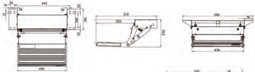
MS1247344 Manual single step 436mm (5.8KG)
