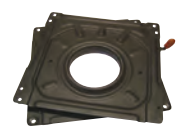
VW T4 swivel 1997 on. Bolt holes on seat box. 426 x 404mm SWVL6R For RH seat SWVL6L For LH seat FASP
