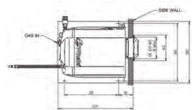
WWH1302 DIMENSIONS
