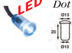
Single push in LED 20mA LFR8878V white LED LFR8878B blue LED IP65 WATERPROOF
